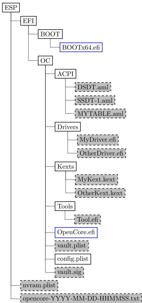
Figure 1. Directory Structure
